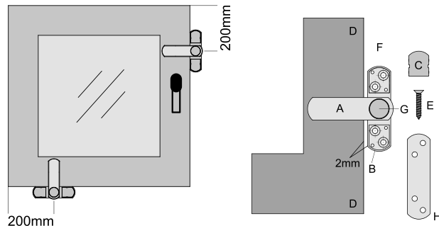
Figure 2: Recommended assembly position
